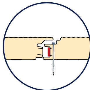
detail montage
