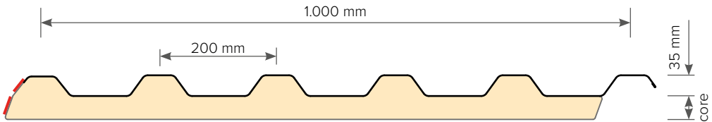
cross section
